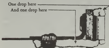
FIGURE 4-60. Oiling the cam follower.
